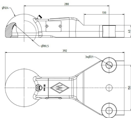
Koblingshode ZKK80-150
