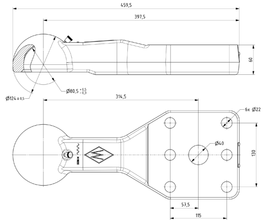
Koblingshode ZKK80-115
