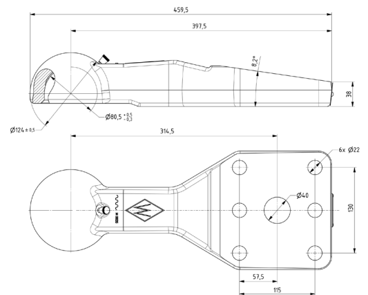
Koblingshode ZKK80-115W
